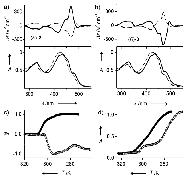
Figure 1. a, b) CD spectra (top) and the corresponding UV absorption spectra (bottom) for ( S )- 2 and ( R )- 3 before (—) and after (.....) UV irradiation at 273 K. c) Normalized CD intensity ( \Phi_n ) at \lambda = 464 nm upon cooling of ( S )- 2 before (●) and after (○) UV irradiation. d) The corresponding normalized absorption spectral changes.
